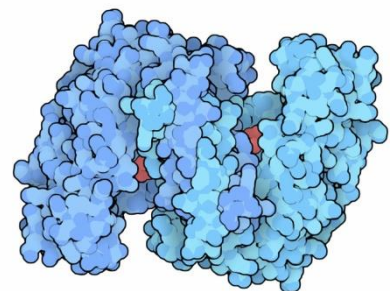
Citratsynthetase Q: www.rcsb.org
