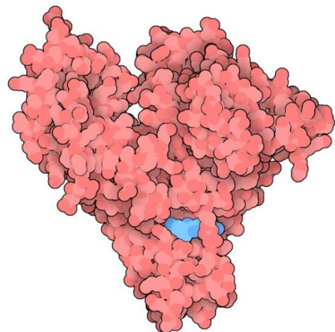
Glucocorticoid-Rezeptor (Molekül-Modell) Q: rcsb.org [Molecule of the Month]
