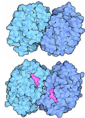
Malatdehydrogenase Q: www.rcsb.org
