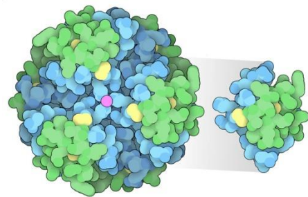
künstlich designtes Insulin (Molekül-Modell) Q: rcsb.org [Molecule of the Month]
