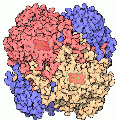
Katalase-Polymer (Molekül-Modell) Q: rcsb.org [Molecule of the Month]
