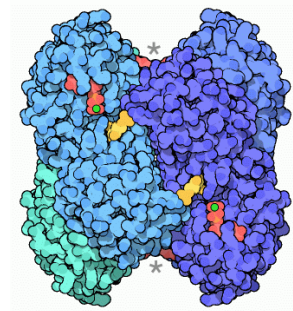
Phosphofructokinase-Tetramer
