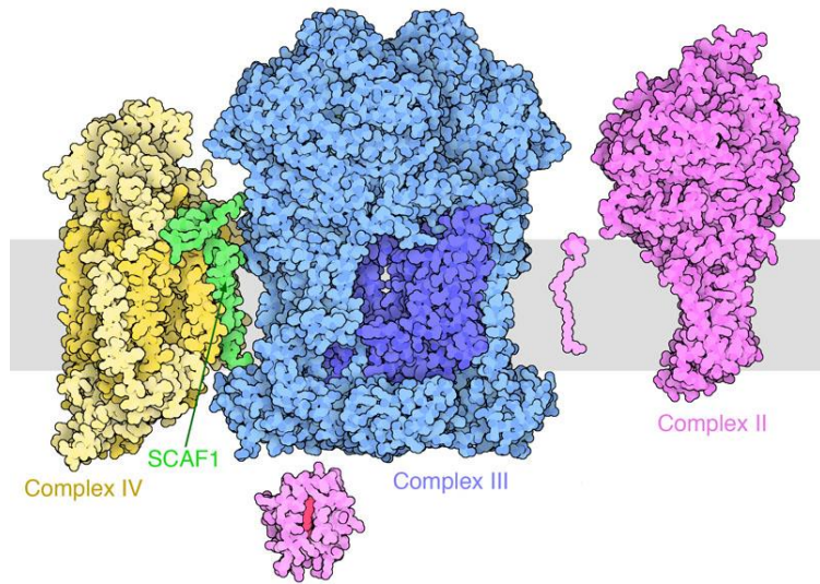
repiratorischer Super-Komplex Q: rcsb.org [Molecule of the Month]
