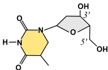
Nucleosid Desoxy-Thymidin
