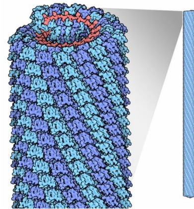
Tabak-Mosaik-Virus
